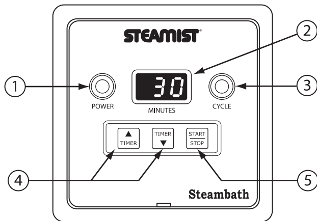
DTC-200 Digital Timer Control
