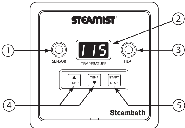
DTC-225 Digital Temperature Control
