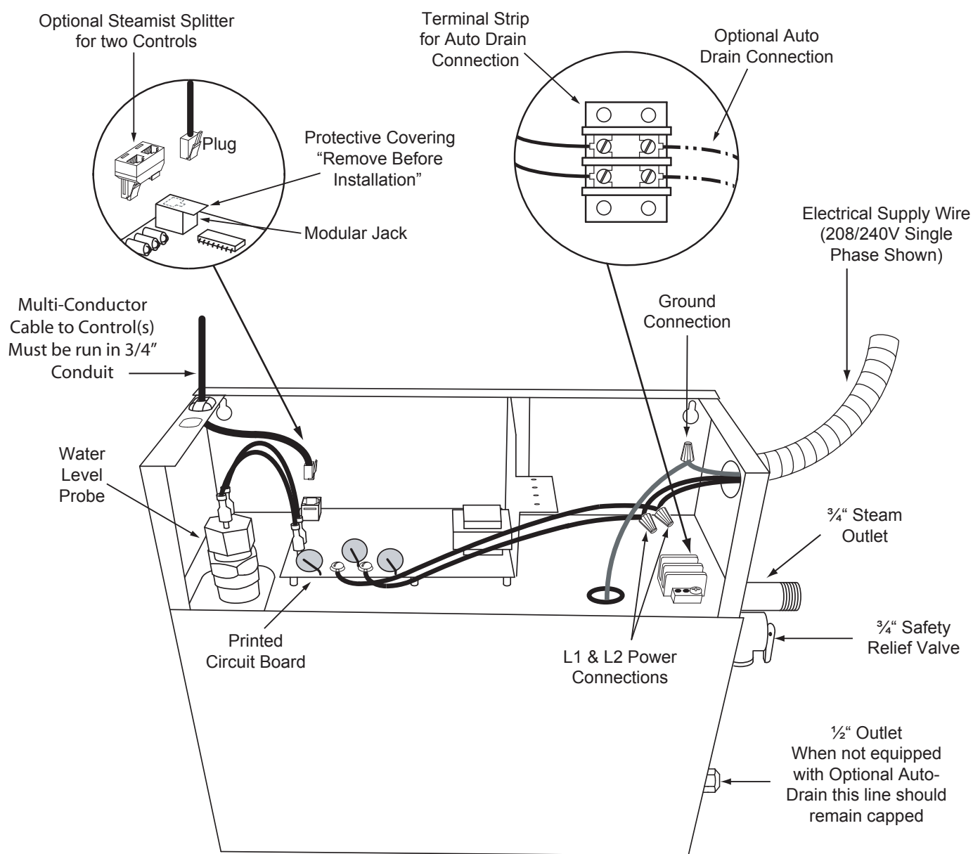
Figure 2: Major Electrical Components
