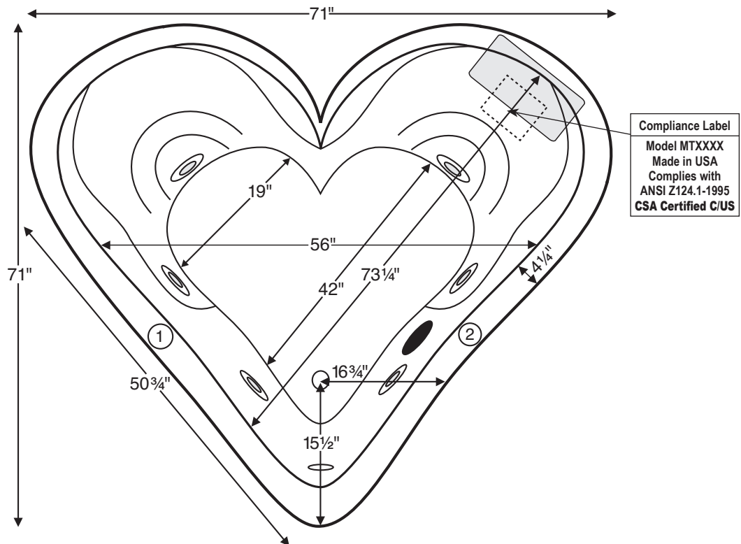
Numbered locations on tub deck are possible Fill-Flush, Hand-Held Shower or Breda locations. Shown with Premium Therapy Package.
