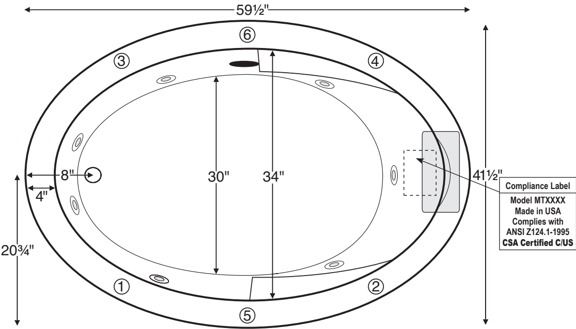
Numbered locations on tub deck are possible Fill-Flush, Hand-Held Shower or Breda locations.
