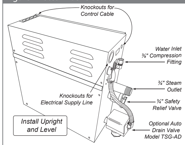
Figure 1 - Steam Generator
