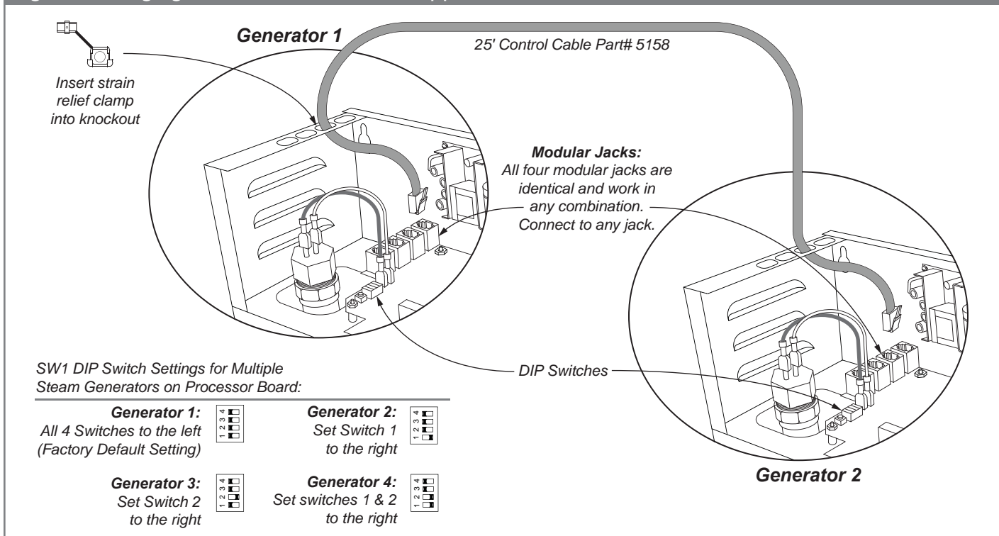
Figure 4 - Typical Installation
