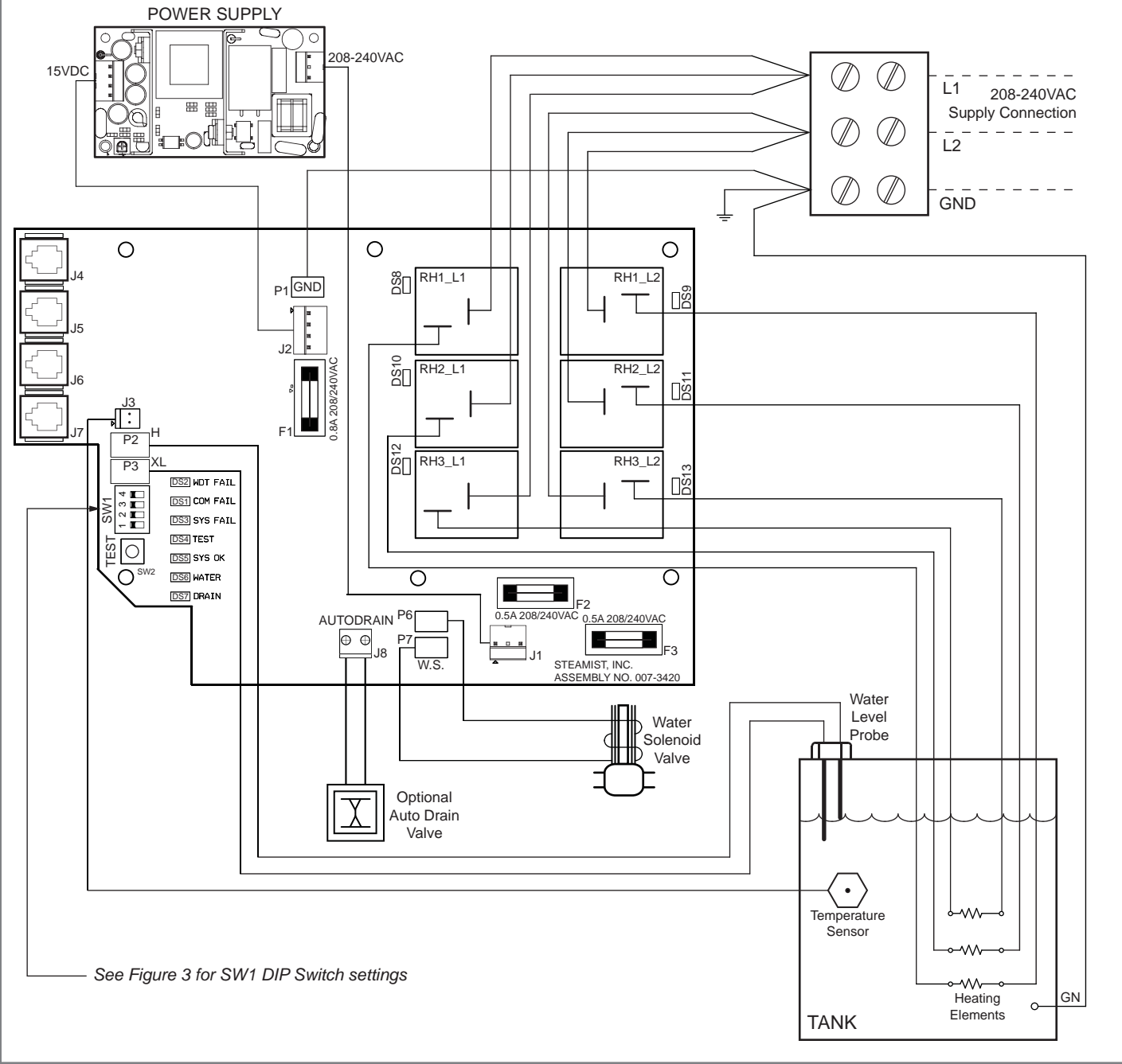
Figure 5 - Wiring Diagram
