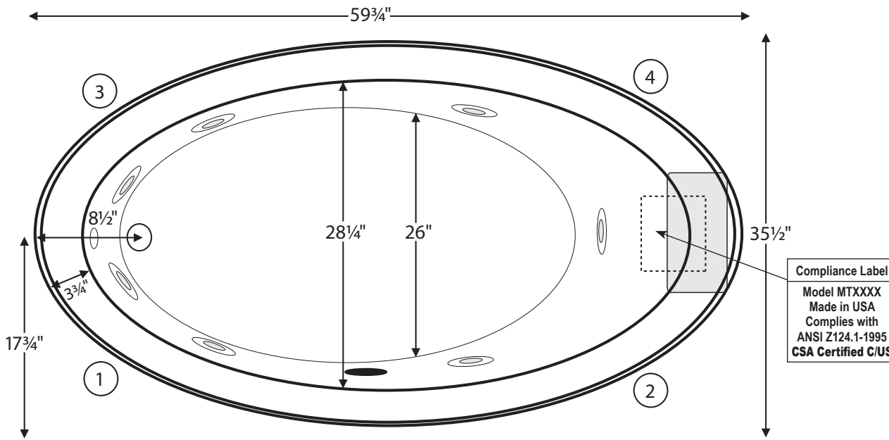
Numbered locations are possible stub-out locations for Fill-Flush, Hand-Held Shower or Breda.
