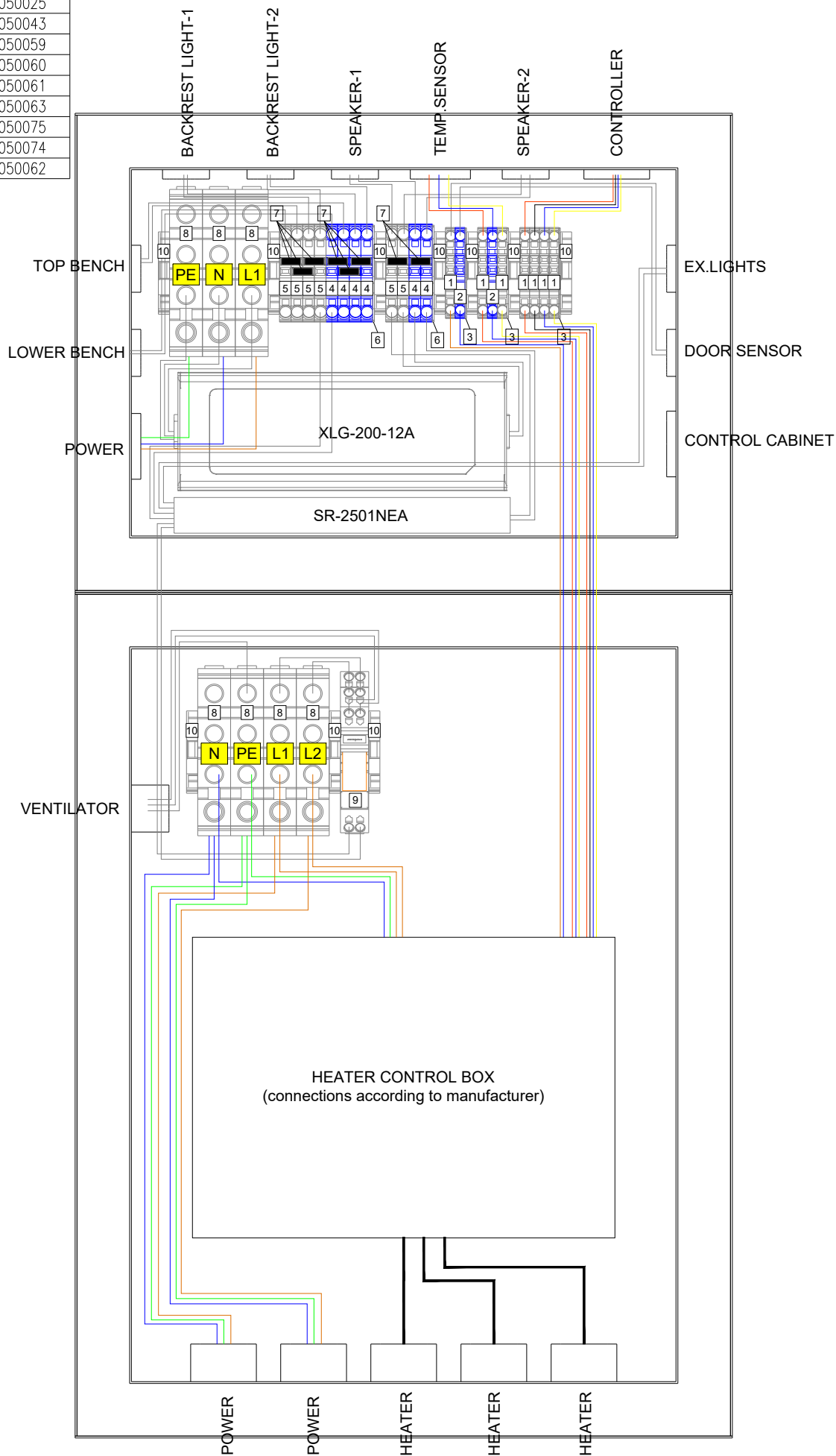
Figure 2. SAUNUM AIRCUBE ONE CONNECTIONS AFTER SAUNA INSTALLATION
