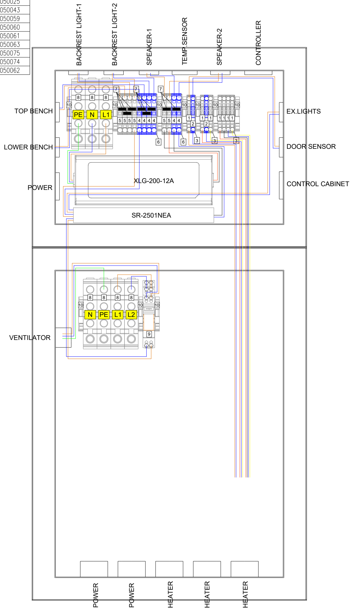
Figure 1. SAUNUM AIRCUBE ONE CONNECTIONS DONE IN FACTORY
