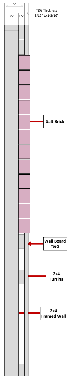
Side View
