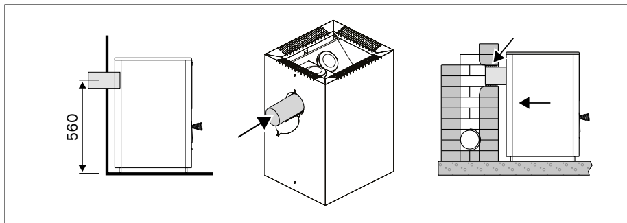
9. Connecting the stove to a masonry flue via the rear connection opening
