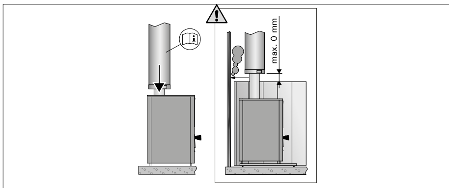
11. Connecting the stove to a Harvia steel chimney
