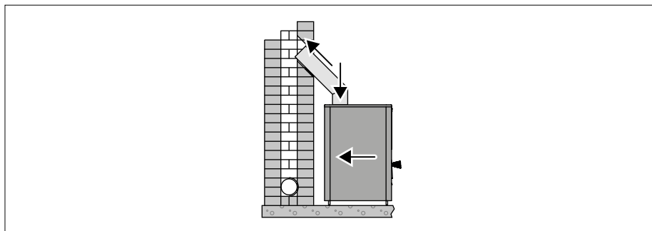
10. Connecting the stove to a masonry flue via the upper connection opening
