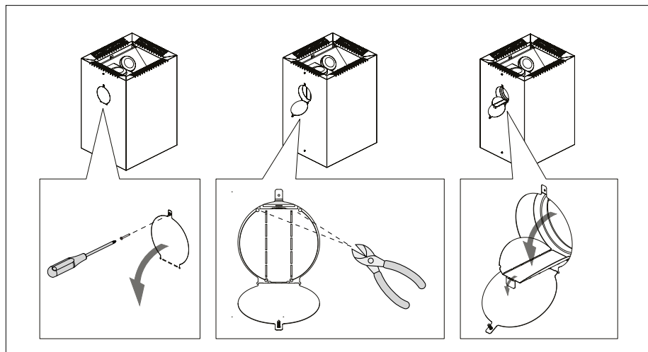
6. Rear connection opening
